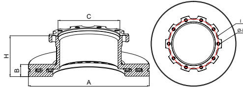
Technical Drawing
