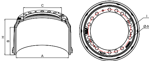
Technical Drawing
