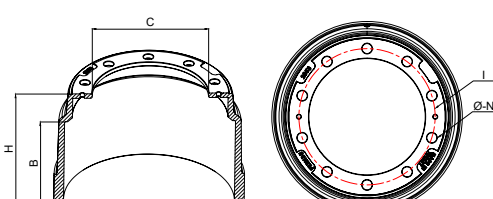
Techinal Drawing
