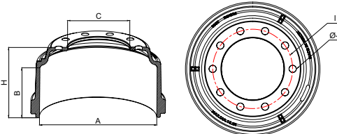
Techinal Drawing
