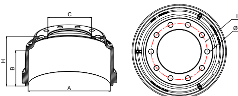
Techinal Drawing
