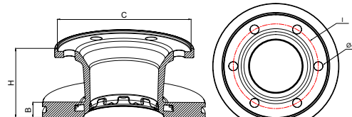
Techinal Drawing
