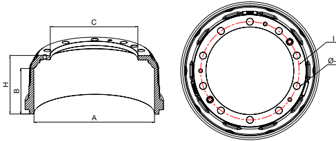
Technical Drawing
