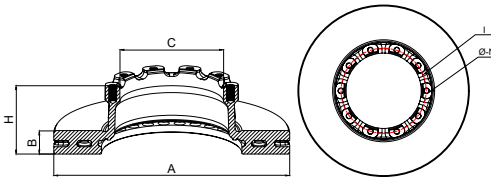
Technical Drawing
