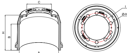
Techinal Drawing
