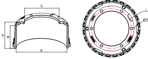
Techinal Drawing
