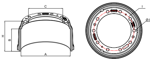
Technical Drawing
