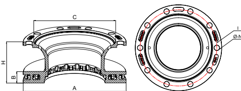
Technical Drawing
