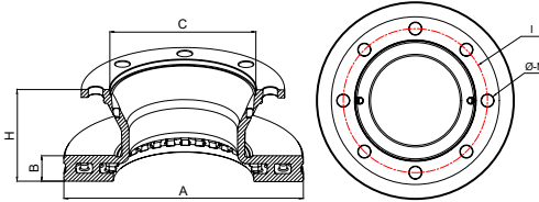
Technical Drawing
