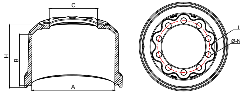
Technical Drawing
