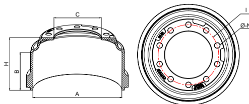
Technical Drawing
