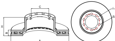
Techinal Drawing
