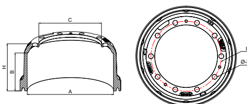
Technical Drawing
