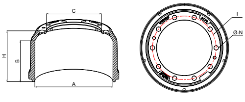
Techinal Drawing
