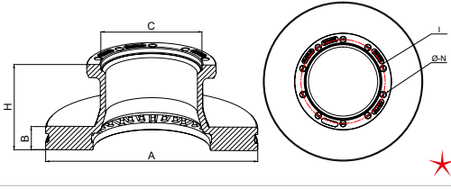
Techinal Drawing
