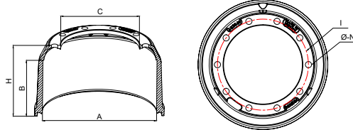
Techinal Drawing
