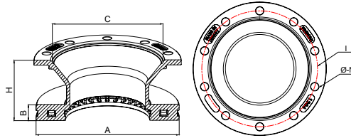
Techinal Drawing
