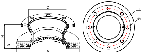
Techinal Drawing
