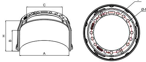
Techinal Drawing
